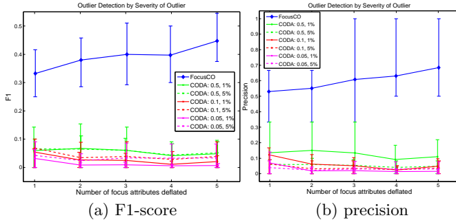
Figure 5: Outlier detection performance by increasing number of deflated focus attributes.
